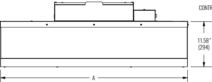
SIDE VIEW 1 - 24"x48" PANEL CRFF-B-ARS, CRFF-B-ARSM
