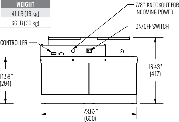
SIDE VIEW 2 - 24"x48" PANEL CRFF-B-ARS, CRFF-B-ARSM
