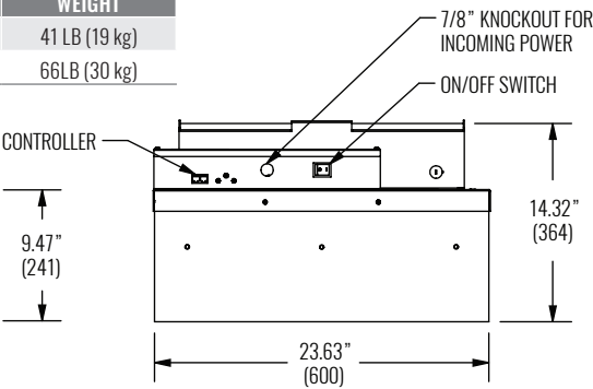
SIDE VIEW 2 - 24"x48" PANEL CRFF-B
