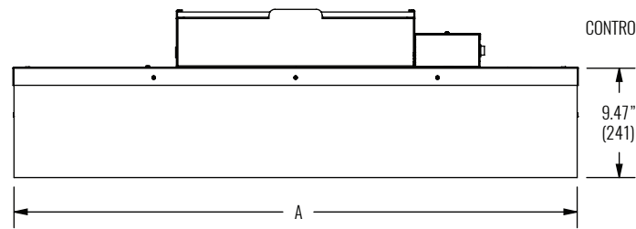
SIDE VIEW 1 - 24"x48" PANEL CRFF-B
