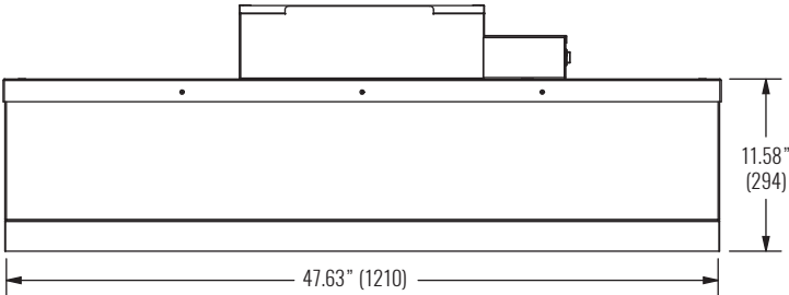
SIDE VIEW 1 - 24"x48" PANEL CRFF-L-ARSM
