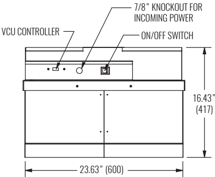
SIDE VIEW 2 - 24"x48" PANEL CRFF-L-ARSM
