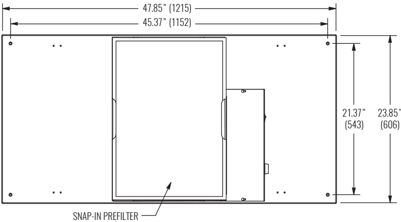
FACE VIEW - 24"x48" PANEL CRFF-L, CRFF-L-ARSM
