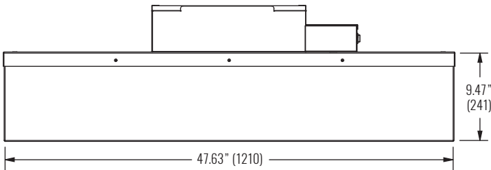
SIDE VIEW 1 - 24"x48" PANEL CRFF-L
