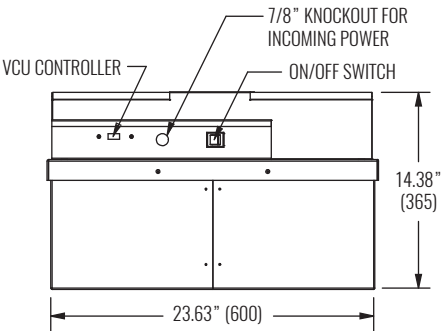
SIDE VIEW 2 - 24"x48" PANEL CRFF-L
