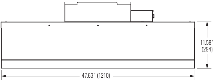
SIDE VIEW 1 - 24"x48" PANEL CRFF-E-ARS, CRFF-E-ARSM
