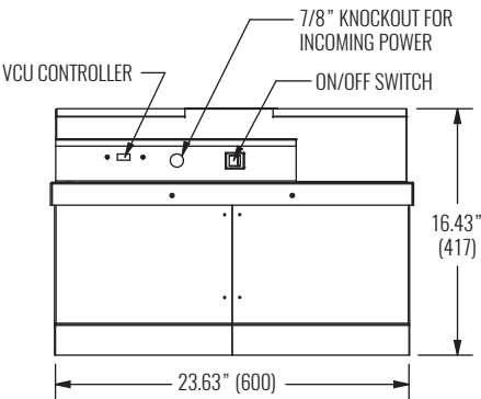
SIDE VIEW 2 - 24"x48" PANEL CRFF-E-ARS, CRFF-E-ARSM
