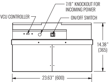
SIDE VIEW 2 - 24"x48" PANEL CRFF-E
