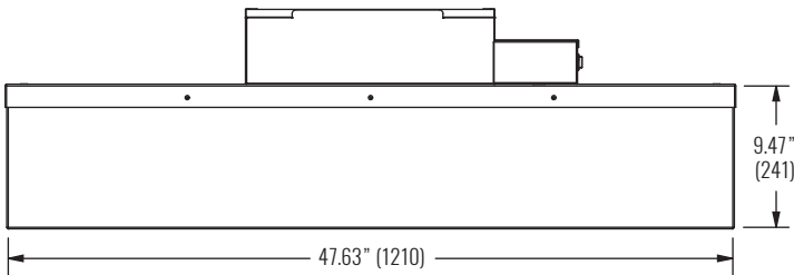
SIDE VIEW 1 - 24"x48" PANEL CRFF-E
