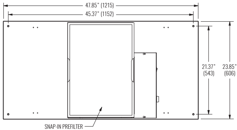
FACE VIEW - 24"x48" PANEL CRFF-E, CRFF-E-ARS, CRFF-E-ARSM
