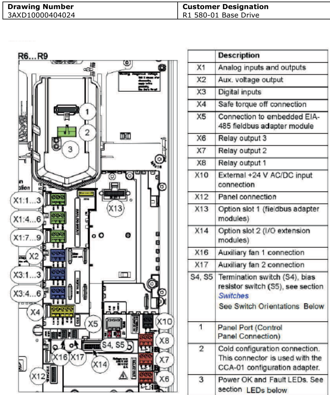
FIGURE 54 - EXTERNAL CONTROL CONNECTION TERMINALS, FRAMES R6...R9
