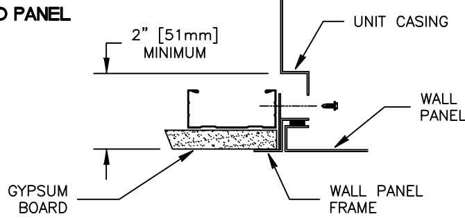
INSTALLATION DETAIL (PARTIAL TOP VIEW)
