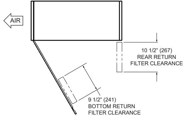
RIGHT VIEW FILTER ACCESS DETAIL TRAP DOOR OPENED
