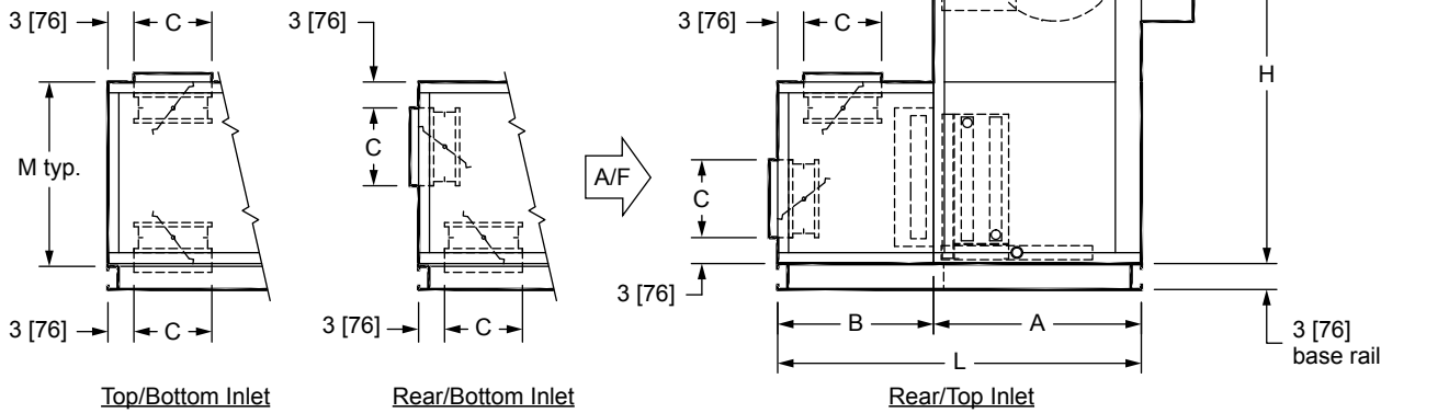
SIDE VIEWS
